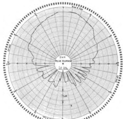
Polar response 10 k.Hz.
