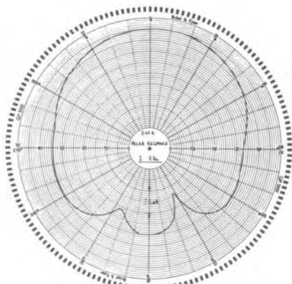
Polar response 1 k.Hz.
